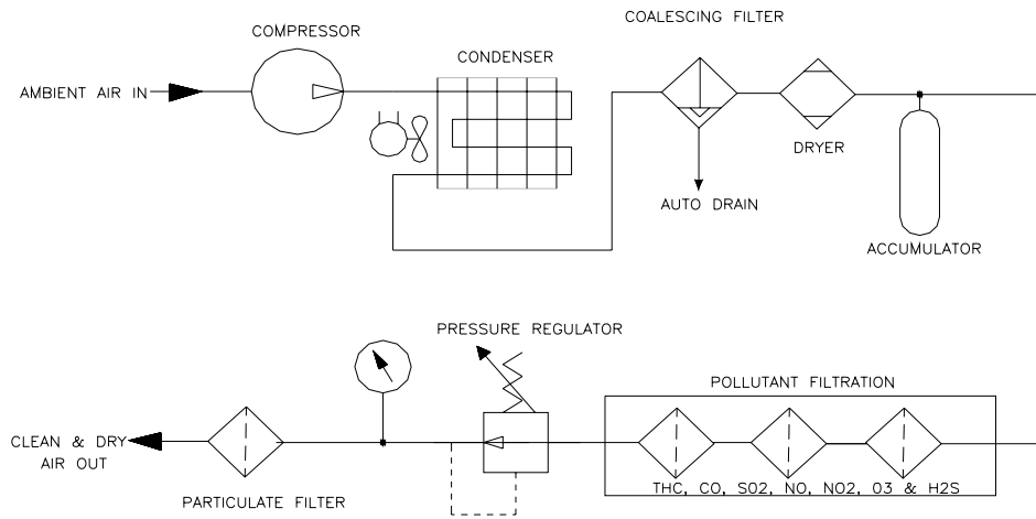
MODEL 7000 P&ID
